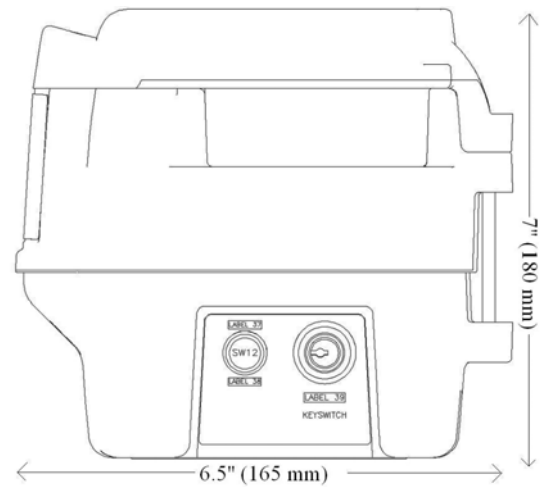
XLTX with Keyswitch and Code Plug
